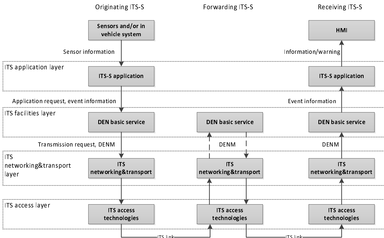
Figure 1: General data flow for ITS-S application supported by the DEN basic service
